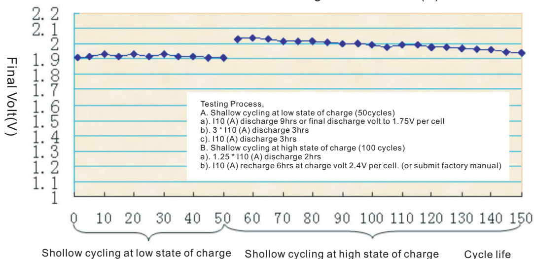
OPzV-350 IEC61427 Testing characteristics(V)
